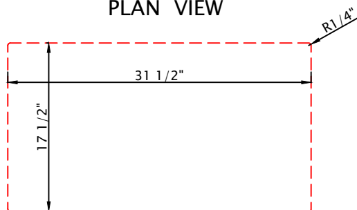
Cut-Out Size
