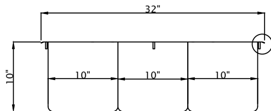
FRONT ELEVATION
